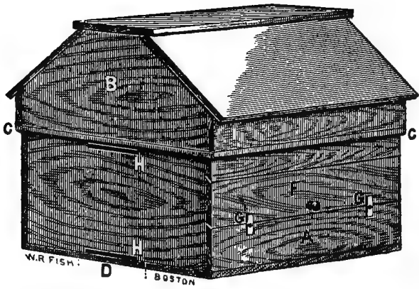
CONTROLLABLE HIVE.—FIGURE 1.
